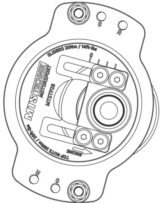
FULL CAMBER +30' CASTER
