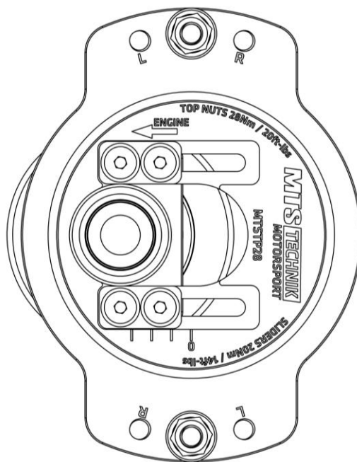
FULL CAMBER OEM CASTER
