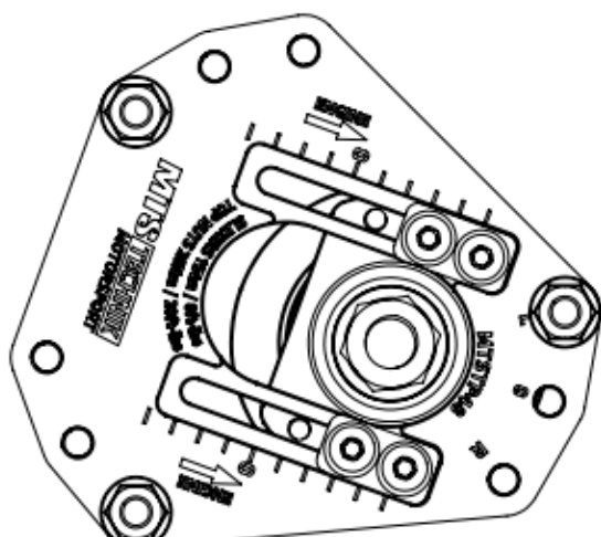
FULL CAMBER +20' CASTER
