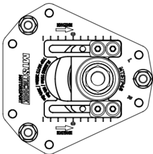
FULL CAMBER OEM CASTER
